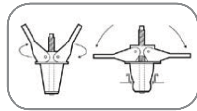
Expansion Plug
